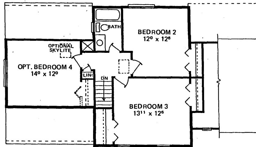
SECOND FLOOR
